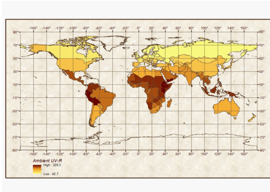
Figure 1: Global distribution of the UV-R variable. Notes: See Andersen et al. (2015) for details on construction of the UV-R index.
