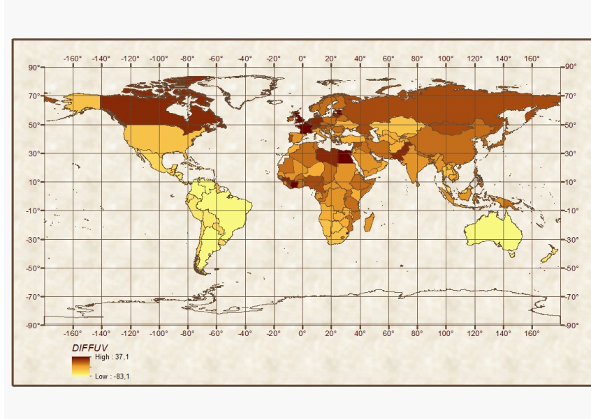
Figure 2: Global map of DIFFUV.
